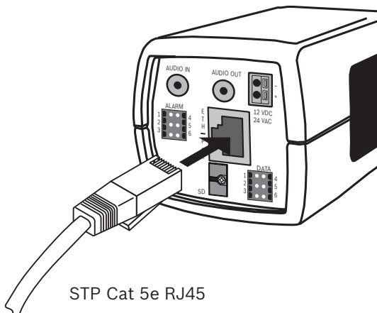
Figure 5.4 Network connection
